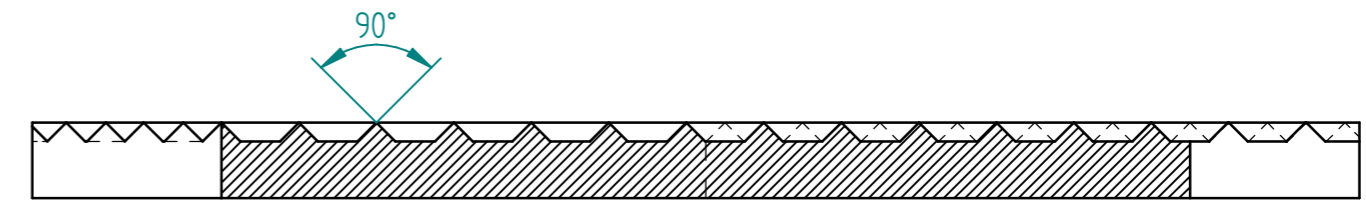
SECTION B-B SCALE 5:1
