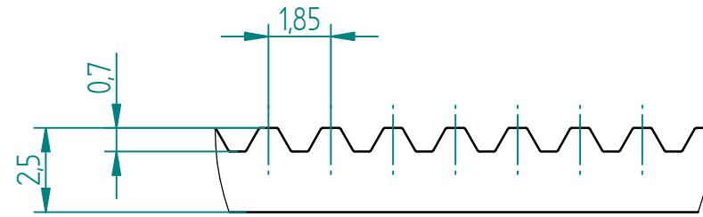
DETAIL B SCALE 5:1
