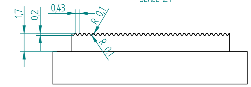
DETAIL C SCALE 5:1
